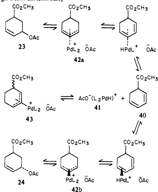
Scheme VI. Interconversion of Cis ( 23 ) and Trans ( 24 ) Acetates through Diene Intermediacy
