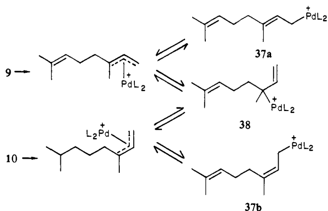
Scheme IV. Mechanism for Interconversion of E and Z Isomers
