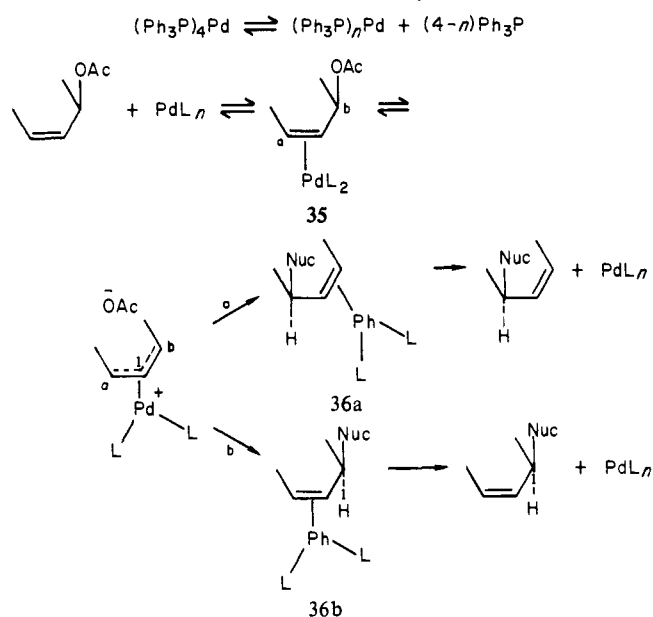
Scheme III. Mechanism of Palladium-Catalyzed Allylic Alkylation
