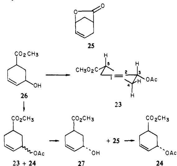
Scheme II. Preparation of ( Z )- and ( E )-3-Acetoxy-5-carbomethoxy-1-cyclohexenes
