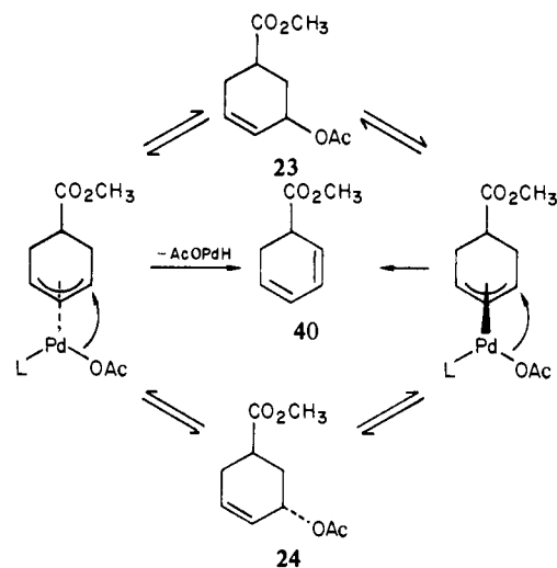
Scheme VII. Interconversion of Cis and Trans Isomers via Internal Transfer
