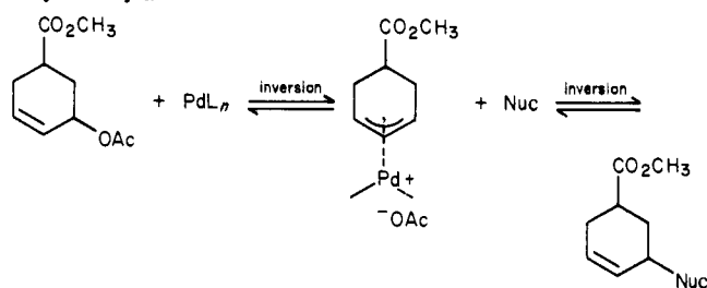
Scheme V. Stereochemistry of Palladium-Catalyzed Allylic Alkylation
