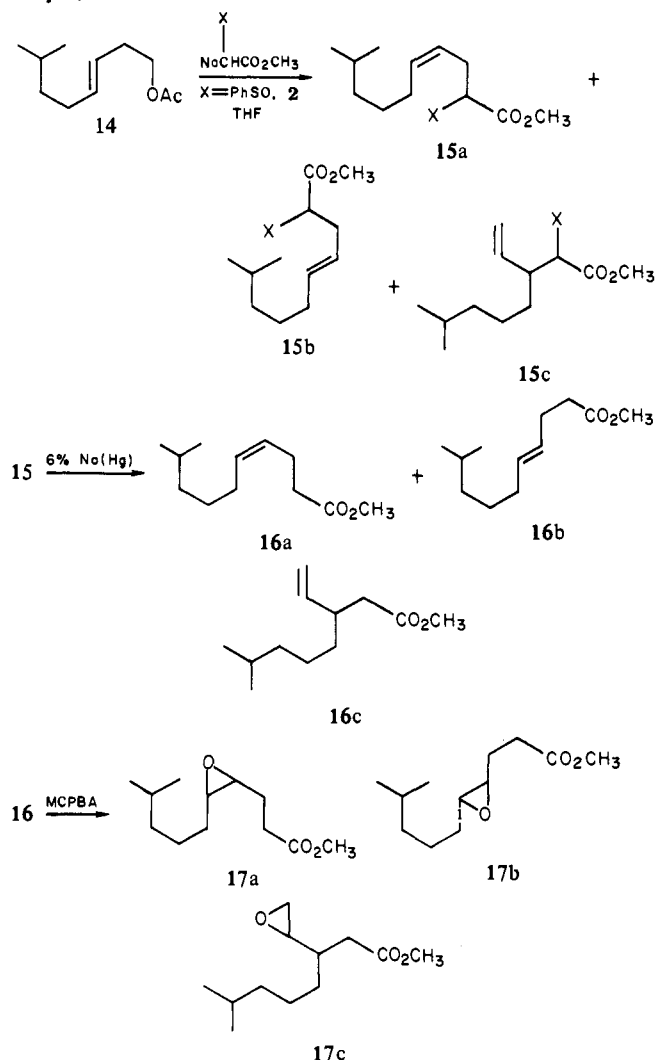
Scheme I. Alkylation of 1-Acetoxy-7-methyl-2-octene ( 14 ) with Methyl Benzenesulfonylacetate. Derivatization of Alkylated Products
